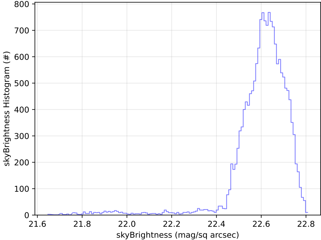
roll_uniform_early_half_accordion1_mjdp0_v3.4_10yrs Yr 1 u band: skyBrightness Histogram
