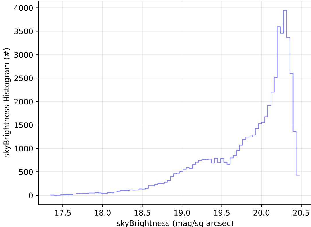
roll_uniform_early_half_accordion1_mjdp0_v3.4_10yrs Yr 1 i band: skyBrightness Histogram
