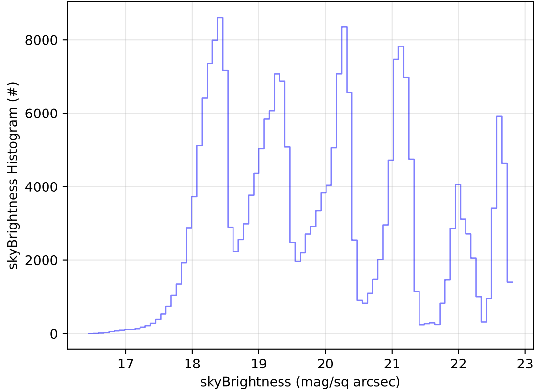
roll_uniform_early_half_accordion1_mjdp0_v3.4_10yrs Yr 1 all bands: skyBrightness Histogram
