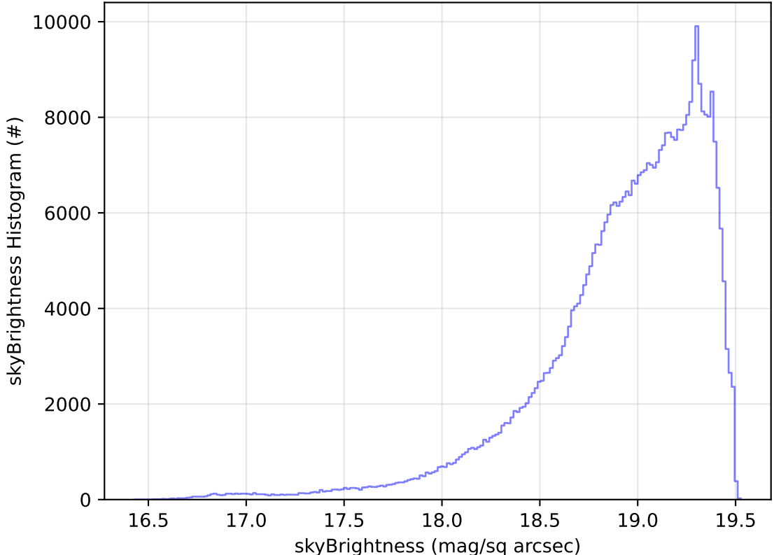
roll_uniform_early_half_accordion1_mjdp0_v3.4_10yrs WFD z band: skyBrightness Histogram
