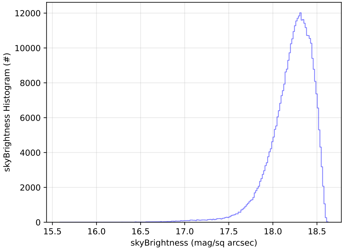
roll_uniform_early_half_accordion1_mjdp0_v3.4_10yrs WFD y band: skyBrightness Histogram
