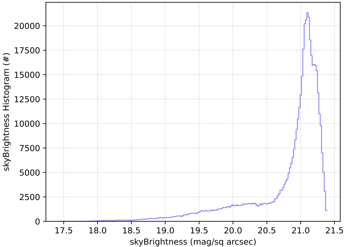
roll_uniform_early_half_accordion1_mjdp0_v3.4_10yrs WFD r band: skyBrightness Histogram
