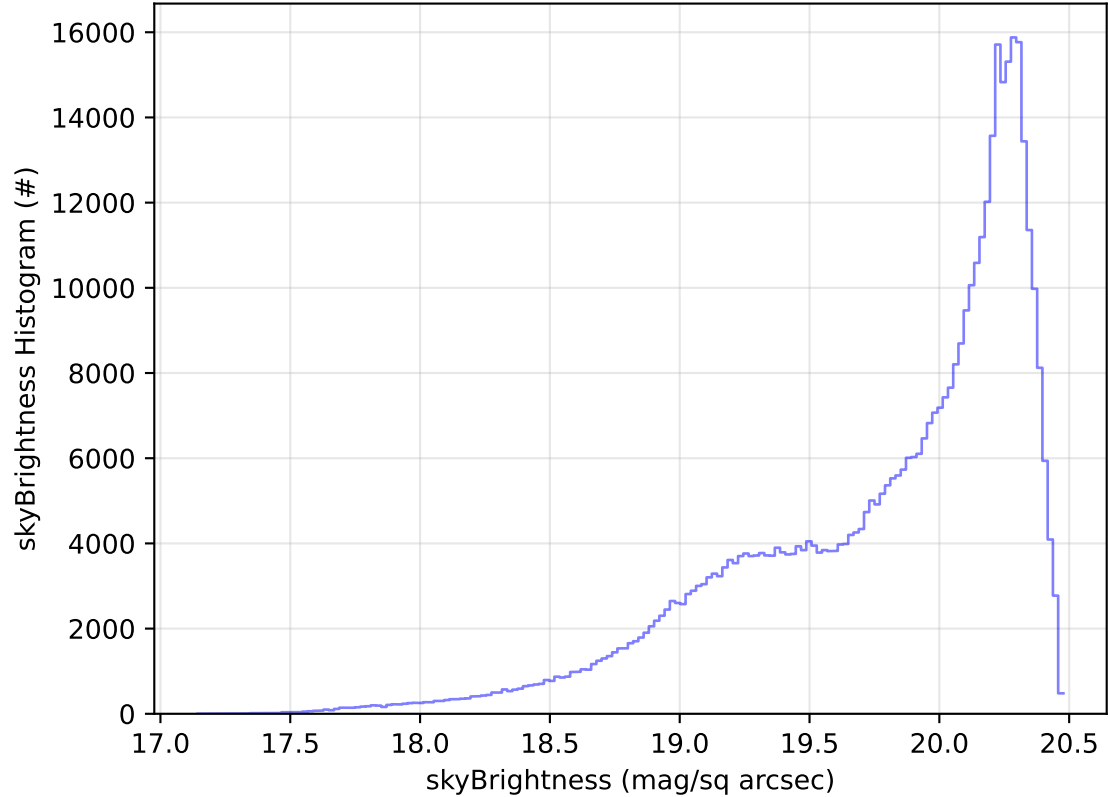
roll_uniform_early_half_accordion1_mjdp0_v3.4_10yrs WFD i band: skyBrightness Histogram
