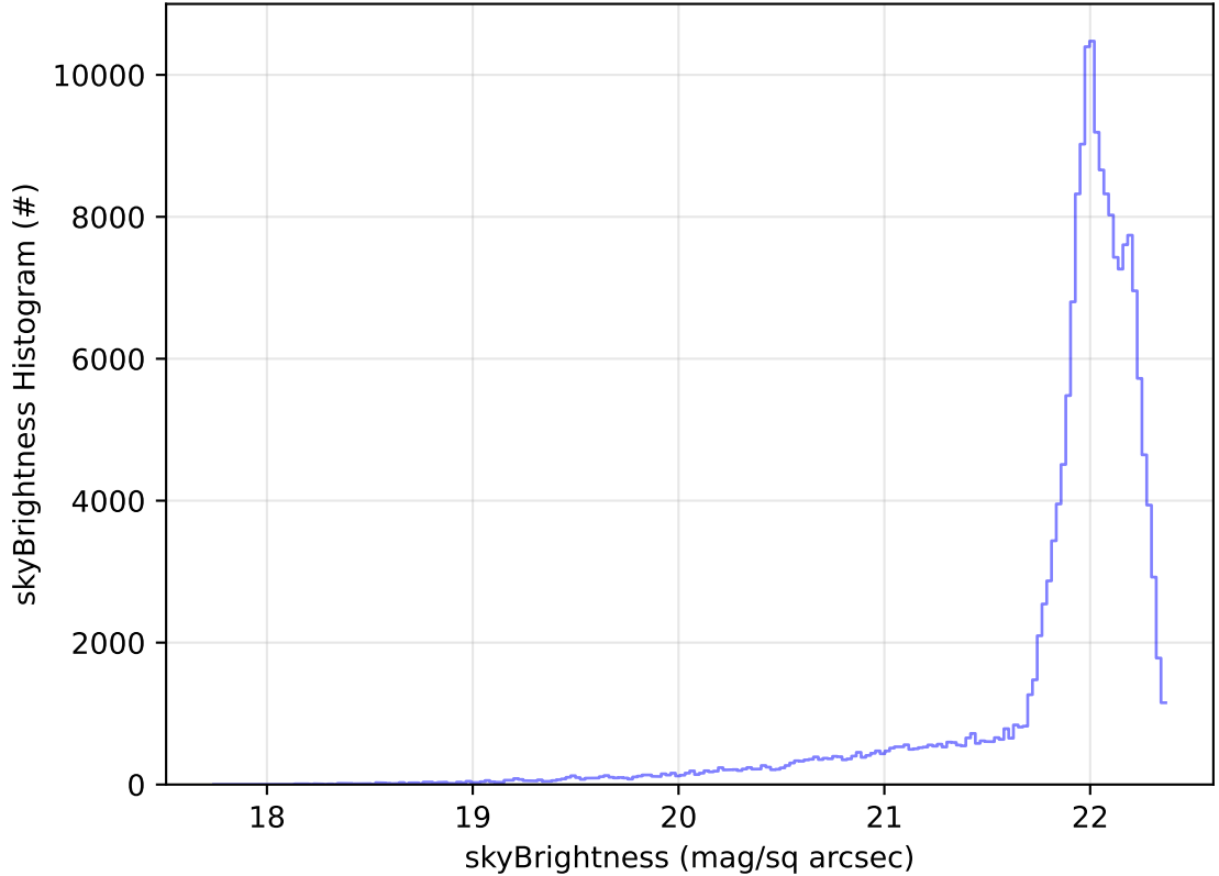
roll_uniform_early_half_accordion1_mjdp0_v3.4_10yrs WFD g band: skyBrightness Histogram
