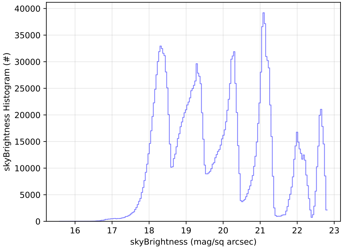
roll_uniform_early_half_accordion1_mjdp0_v3.4_10yrs WFD all bands: skyBrightness Histogram
