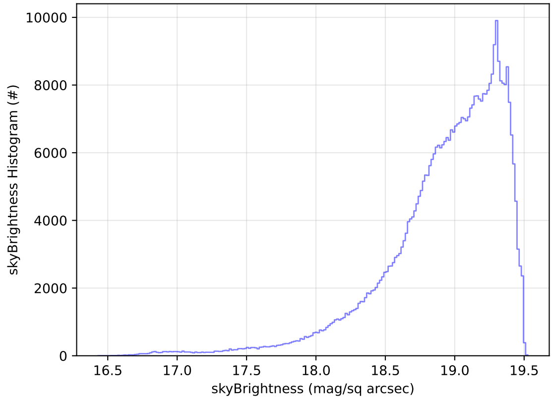
roll_uniform_early_half_accordion1_mjdp0_v3.4_10yrs All sky z band: skyBrightness Histogram
