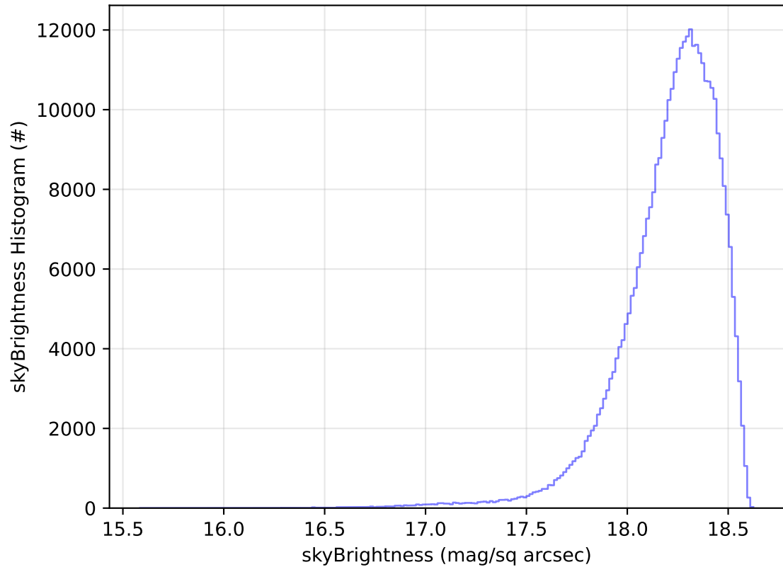
roll_uniform_early_half_accordion1_mjdp0_v3.4_10yrs All sky y band: skyBrightness Histogram
