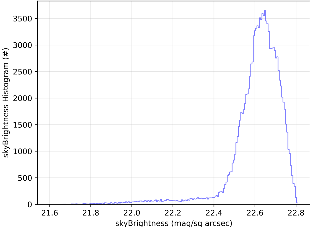
roll_uniform_early_half_accordion1_mjdp0_v3.4_10yrs All sky u band: skyBrightness Histogram
