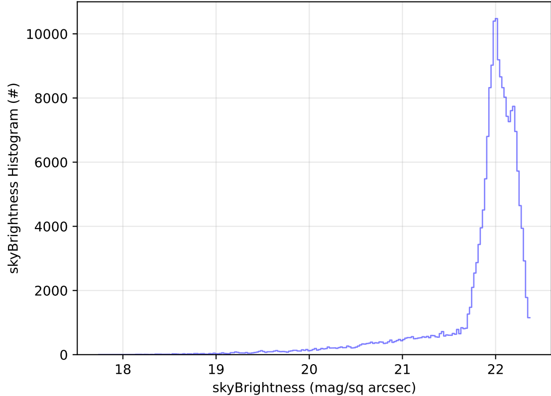
roll_uniform_early_half_accordion1_mjdp0_v3.4_10yrs All sky g band: skyBrightness Histogram
