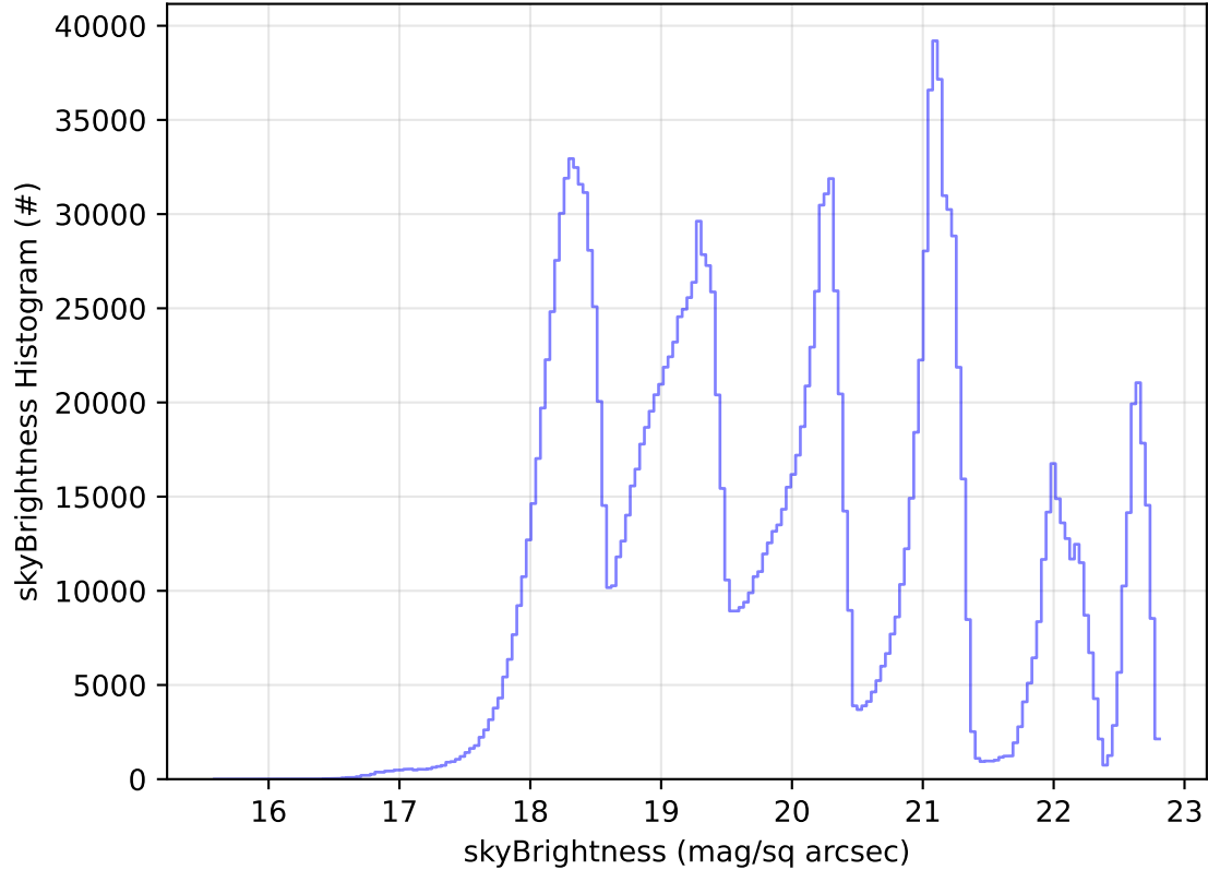
roll_uniform_early_half_accordion1_mjdp0_v3.4_10yrs All sky all bands: skyBrightness Histogram
