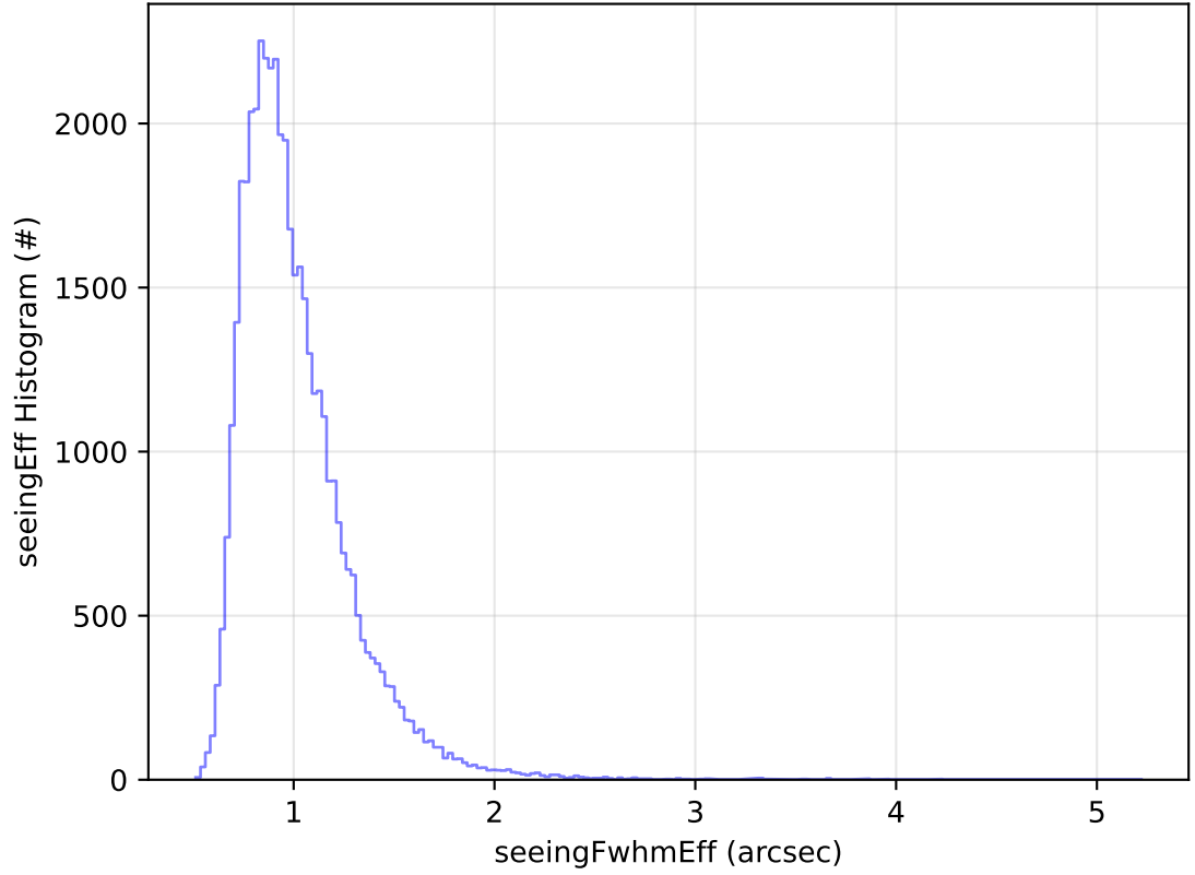
roll_uniform_early_half_accordion1_mjdp0_v3.4_10yrs Yr 1 z band: seeingEff Histogram
