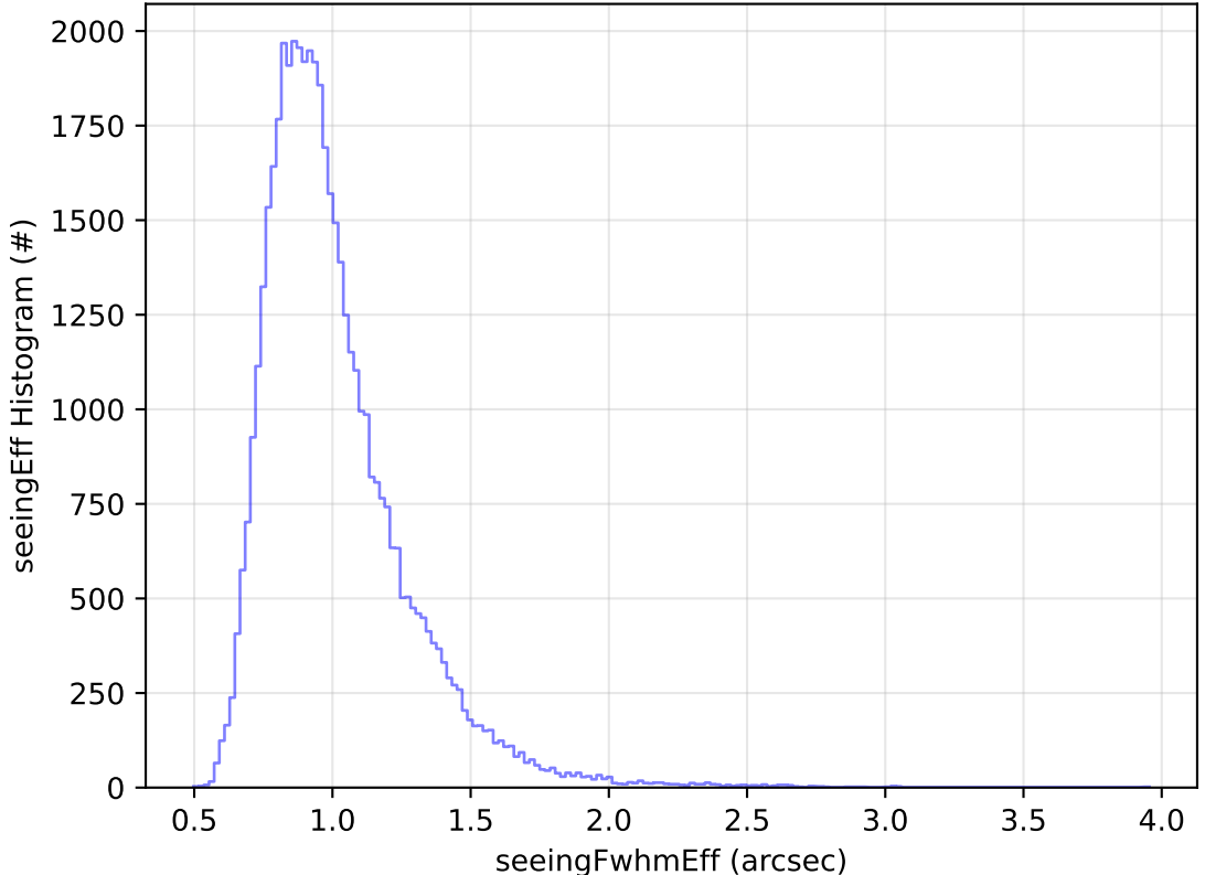
roll_uniform_early_half_accordion1_mjdp0_v3.4_10yrs Yr 1 y band: seeingEff Histogram
