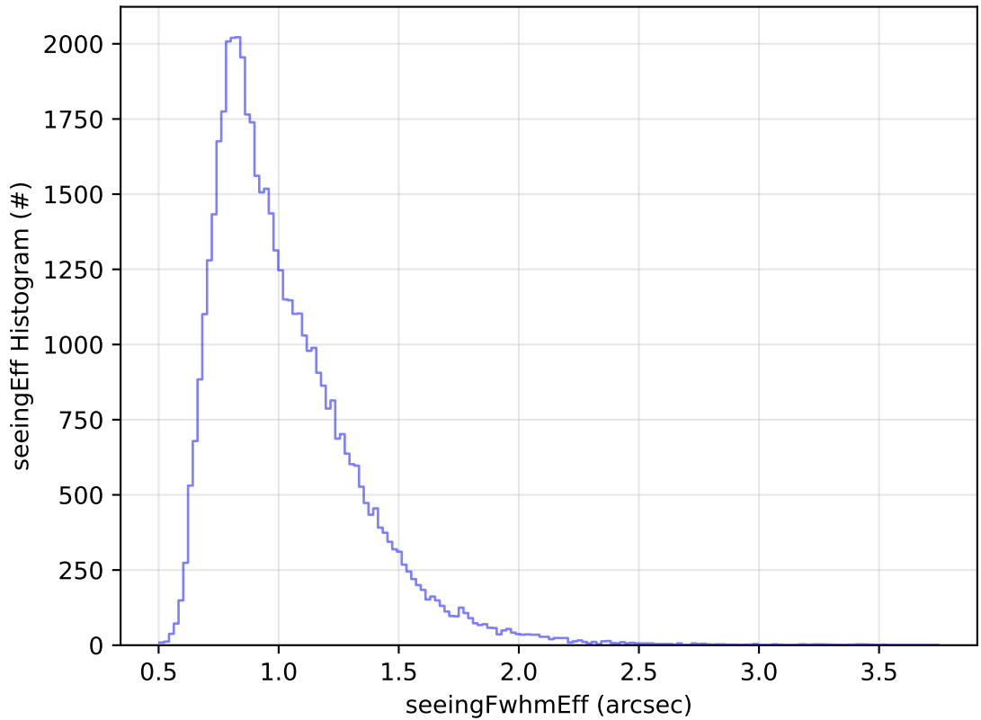
roll_uniform_early_half_accordion1_mjdp0_v3.4_10yrs Yr 1 r band: seeingEff Histogram
