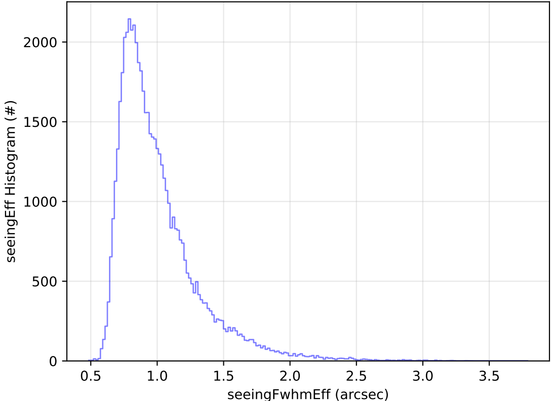
roll_uniform_early_half_accordion1_mjdp0_v3.4_10yrs Yr 1 i band: seeingEff Histogram
