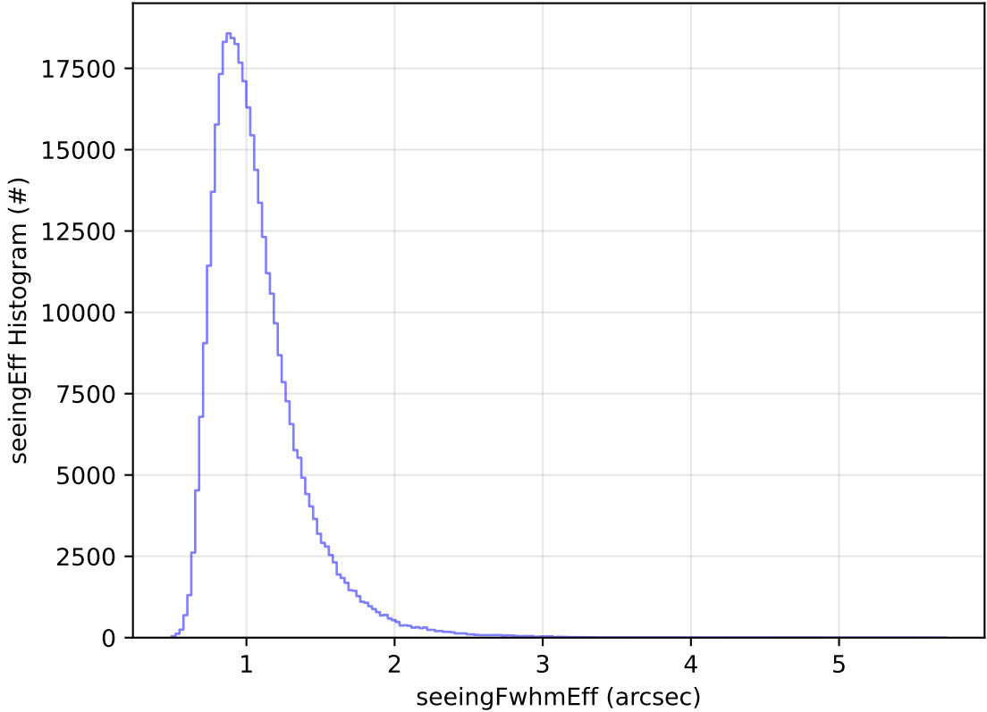
roll_uniform_early_half_accordion1_mjdp0_v3.4_10yrs WFD y band: seeingEff Histogram
