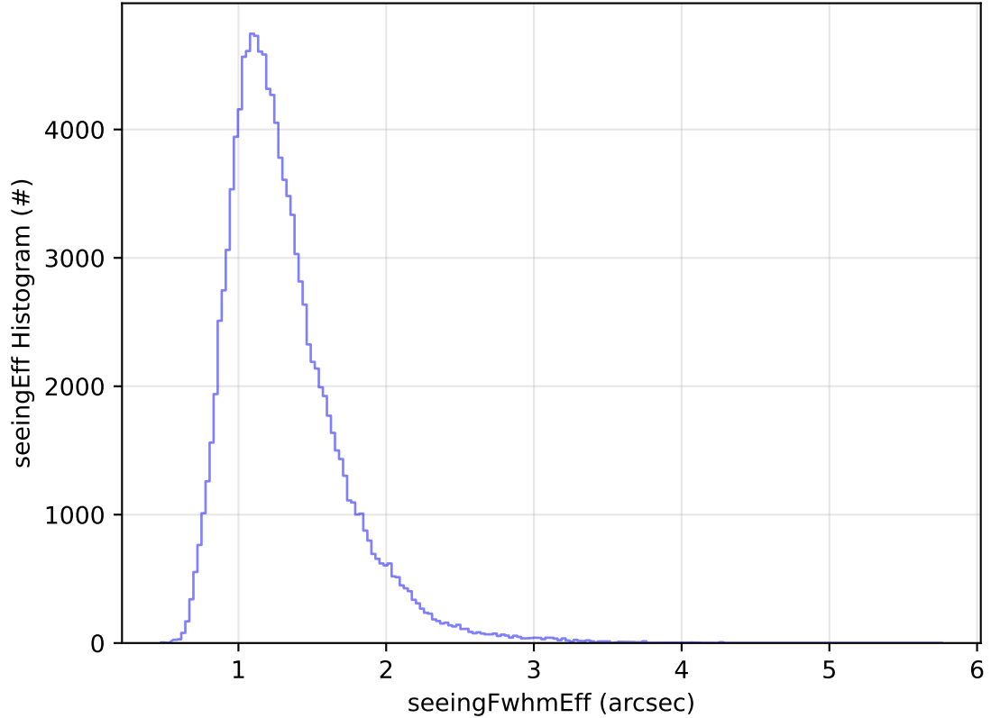
roll_uniform_early_half_accordion1_mjdp0_v3.4_10yrs WFD u band: seeingEff Histogram
