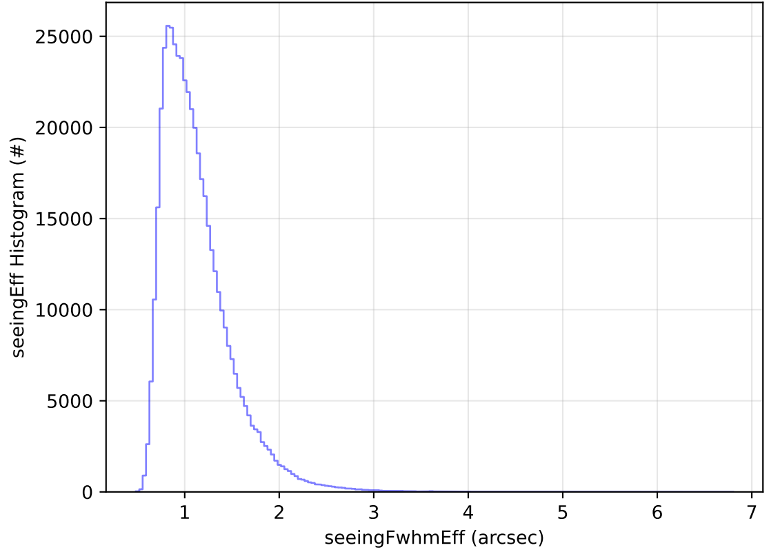
roll_uniform_early_half_accordion1_mjdp0_v3.4_10yrs WFD r band: seeingEff Histogram
