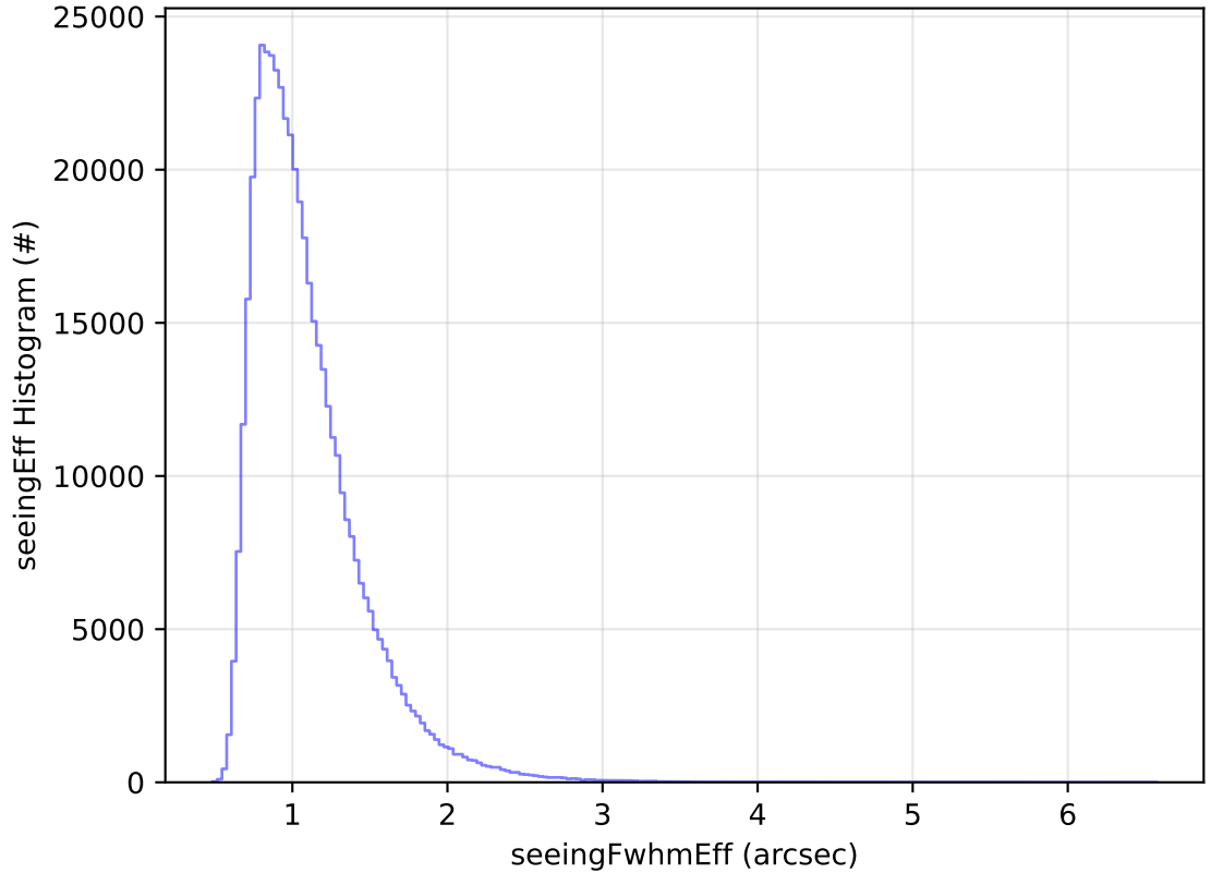
roll_uniform_early_half_accordion1_mjdp0_v3.4_10yrs WFD i band: seeingEff Histogram
