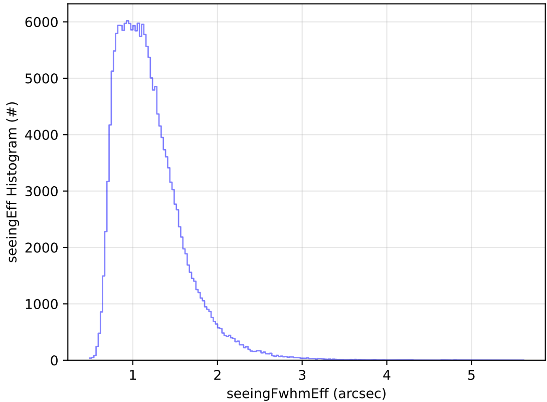
roll_uniform_early_half_accordion1_mjdp0_v3.4_10yrs WFD g band: seeingEff Histogram
