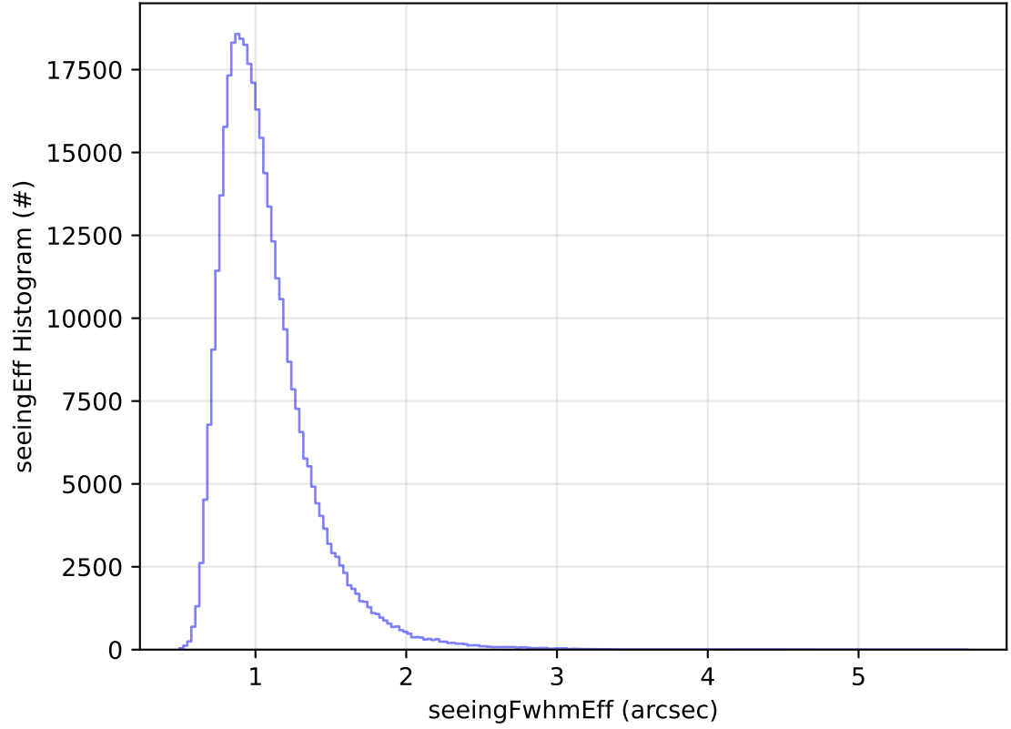
roll_uniform_early_half_accordion1_mjdp0_v3.4_10yrs All sky y band: seeingEff Histogram
