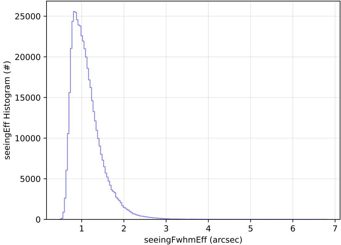
roll_uniform_early_half_accordion1_mjdp0_v3.4_10yrs All sky r band: seeingEff Histogram
