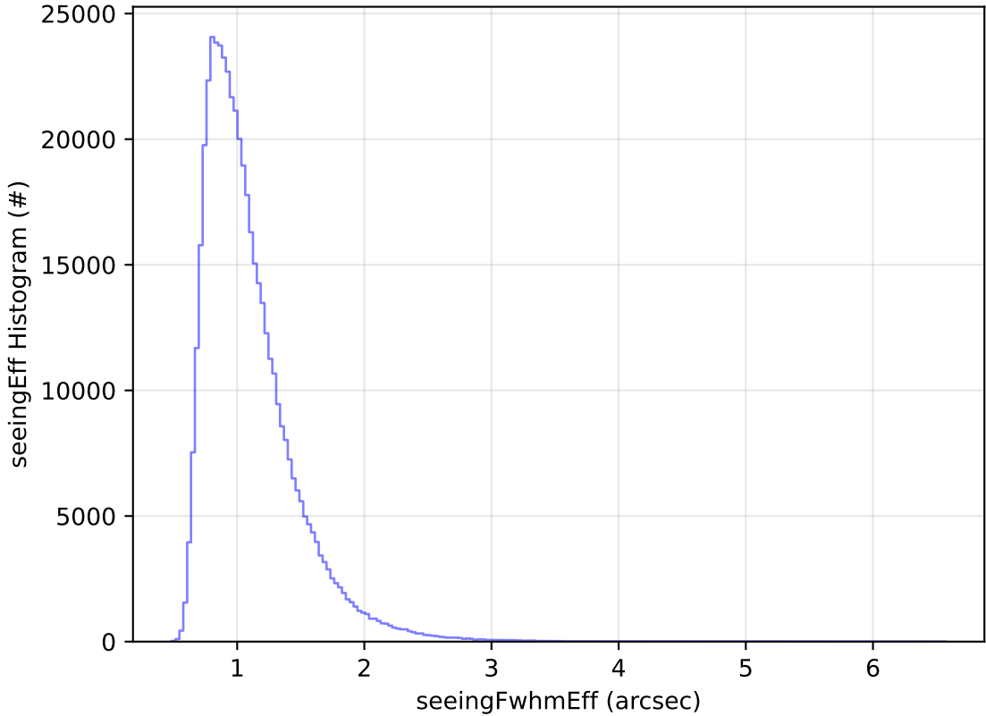
roll_uniform_early_half_accordion1_mjdp0_v3.4_10yrs All sky i band: seeingEff Histogram
