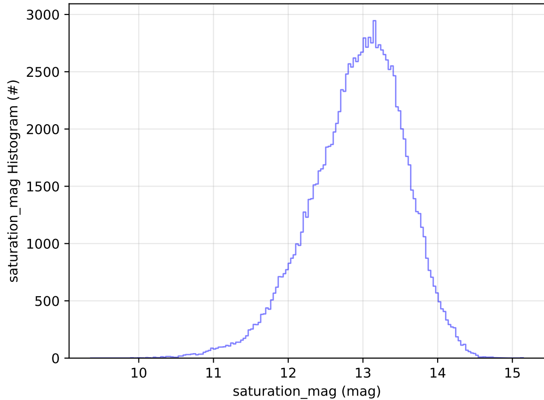
roll_uniform_early_half_accordion1_mjdp0_v3.4_10yrs WFD u band: saturation_mag Histogram
