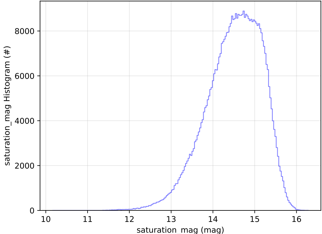
roll_uniform_early_half_accordion1_mjdp0_v3.4_10yrs WFD r band: saturation_mag Histogram
