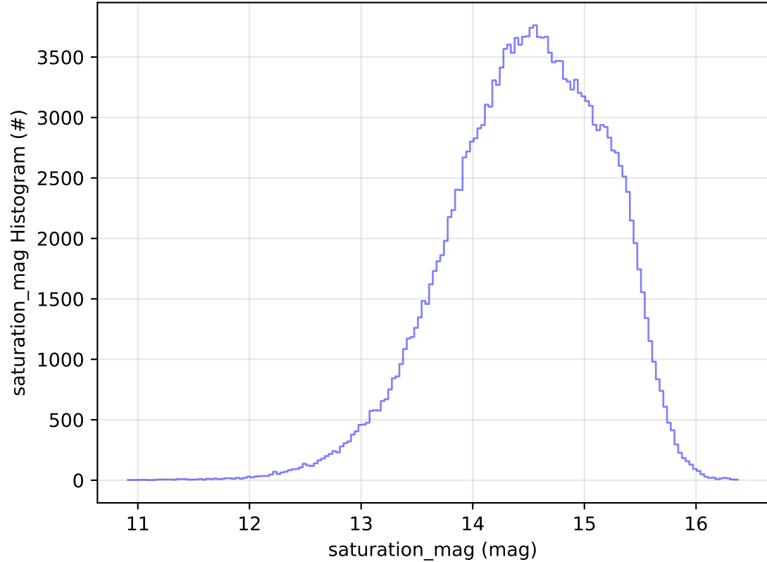
roll_uniform_early_half_accordion1_mjdp0_v3.4_10yrs WFD g band: saturation_mag Histogram
