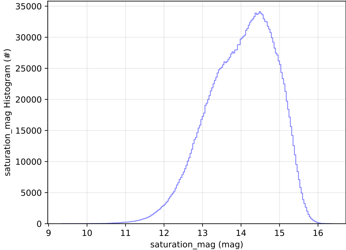
roll_uniform_early_half_accordion1_mjdp0_v3.4_10yrs WFD all bands: saturation_mag Histogram
