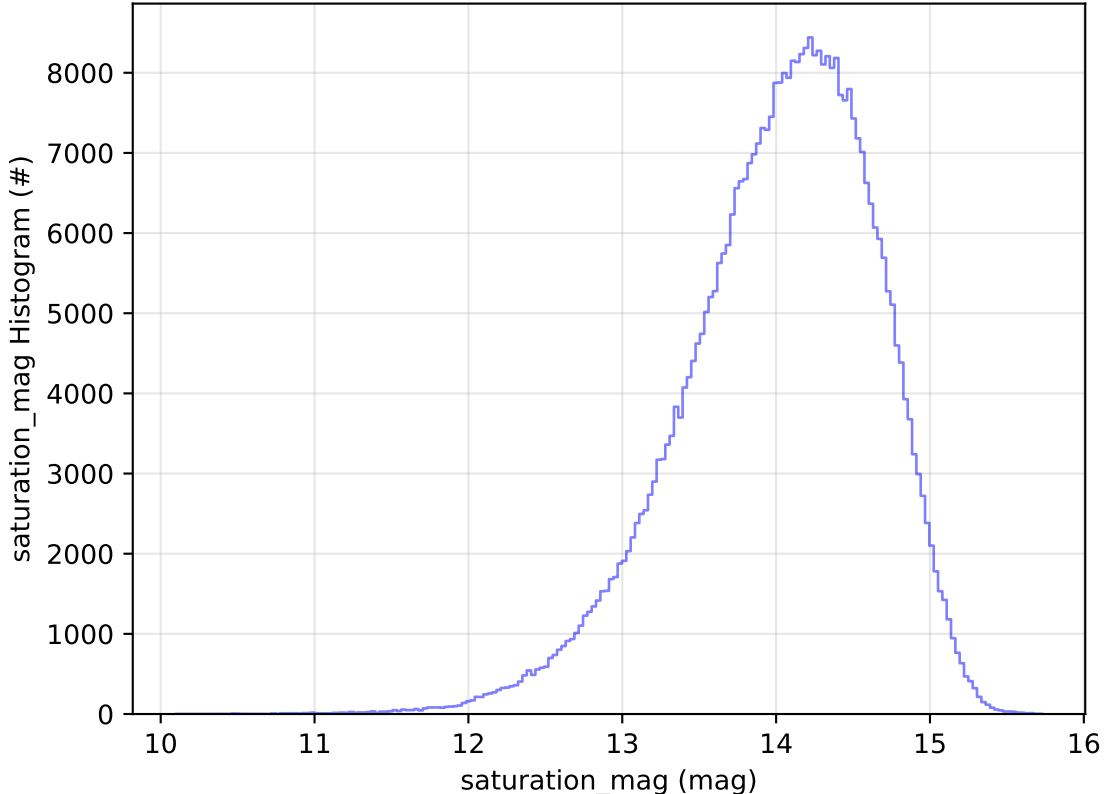
roll_uniform_early_half_accordion1_mjdp0_v3.4_10yrs All sky z band: saturation_mag Histogram
