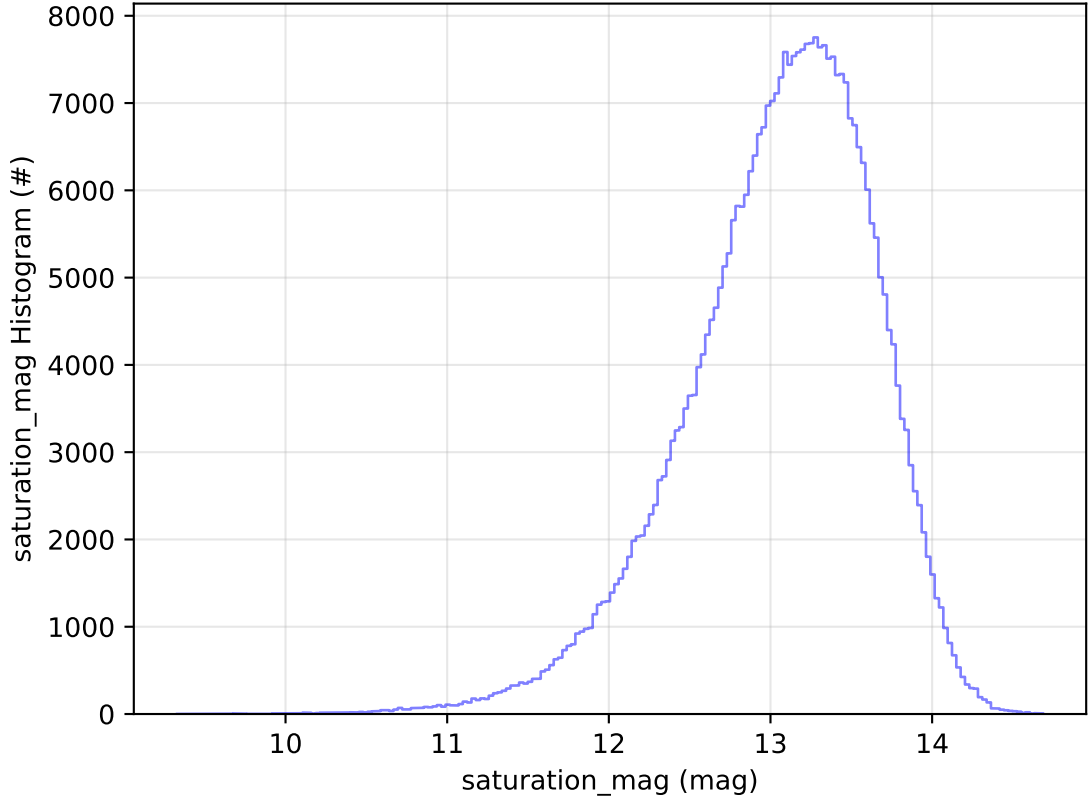
roll_uniform_early_half_accordion1_mjdp0_v3.4_10yrs All sky y band: saturation_mag Histogram
