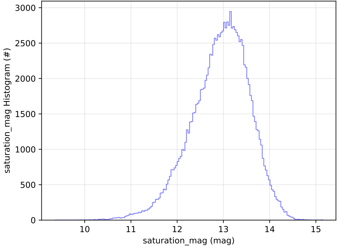
roll_uniform_early_half_accordion1_mjdp0_v3.4_10yrs All sky u band: saturation_mag Histogram
