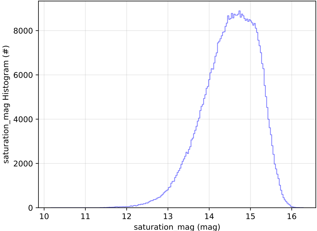
roll_uniform_early_half_accordion1_mjdp0_v3.4_10yrs All sky r band: saturation_mag Histogram
