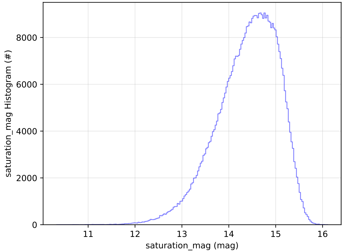
roll_uniform_early_half_accordion1_mjdp0_v3.4_10yrs All sky i band: saturation_mag Histogram
