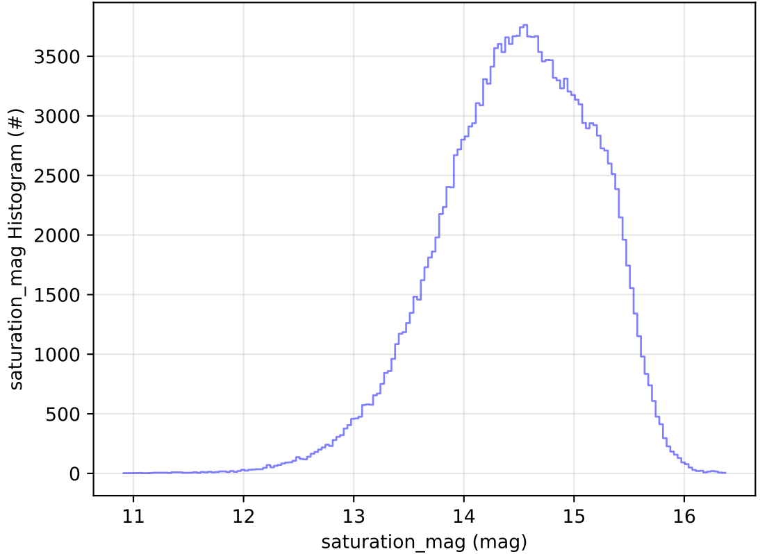
roll_uniform_early_half_accordion1_mjdp0_v3.4_10yrs All sky g band: saturation_mag Histogram
