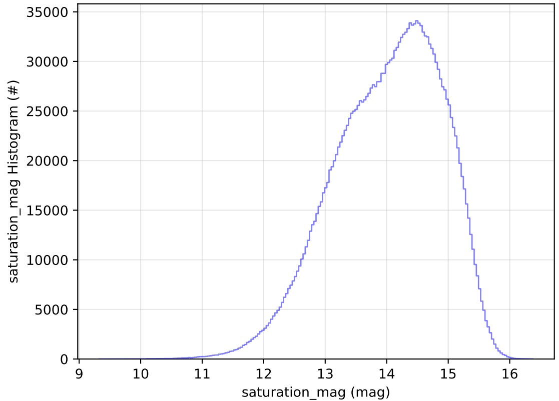
roll_uniform_early_half_accordion1_mjdp0_v3.4_10yrs All sky all bands: saturation_mag Histogram
