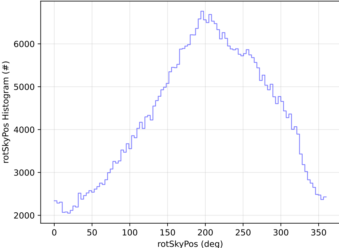
roll_uniform_early_half_accordion1_mjdp0_v3.4_10yrs WFD z band: rotSkyPos Histogram
