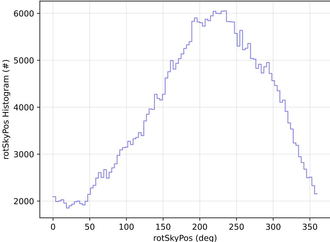
roll_uniform_early_half_accordion1_mjdp0_v3.4_10yrs WFD y band: rotSkyPos Histogram
