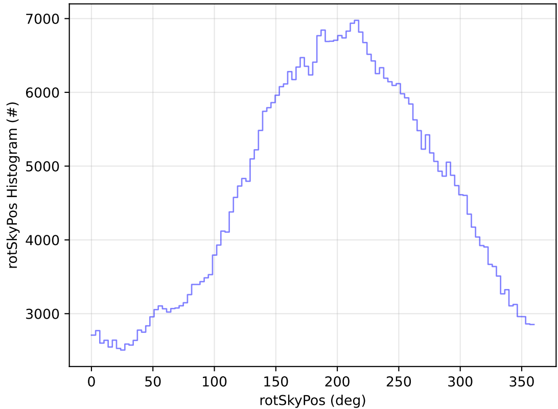
roll_uniform_early_half_accordion1_mjdp0_v3.4_10yrs WFD r band: rotSkyPos Histogram
