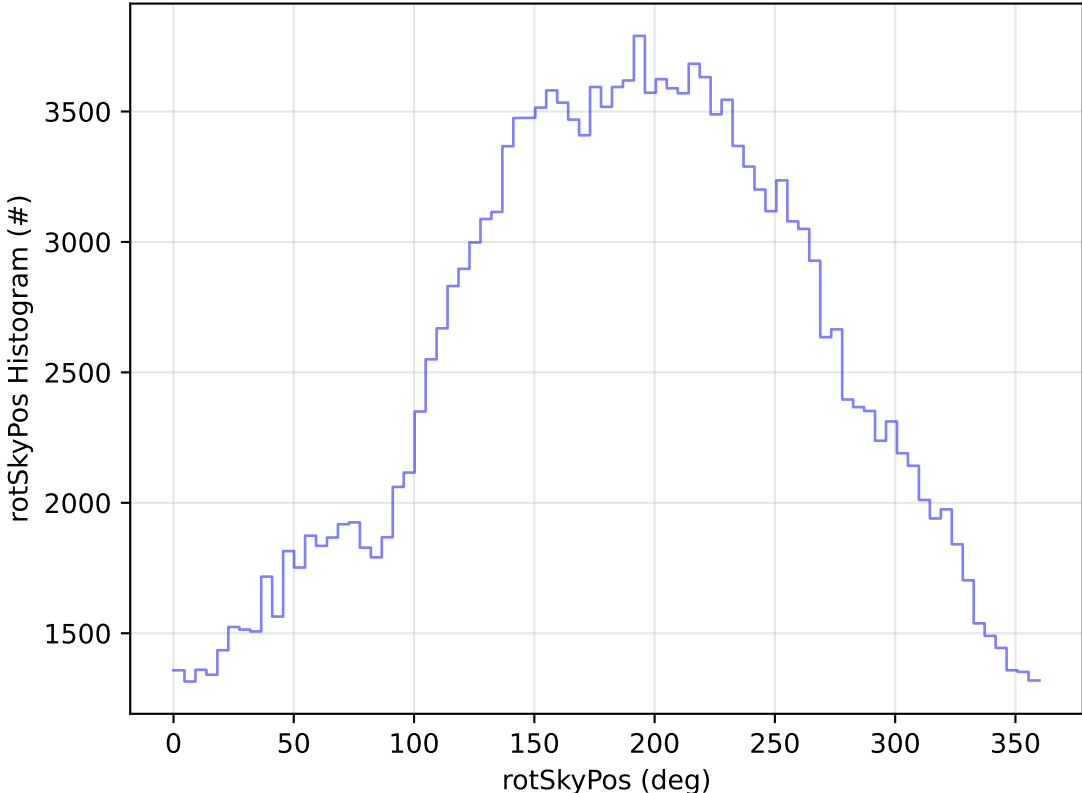
roll_uniform_early_half_accordion1_mjdp0_v3.4_10yrs WFD g band: rotSkyPos Histogram
