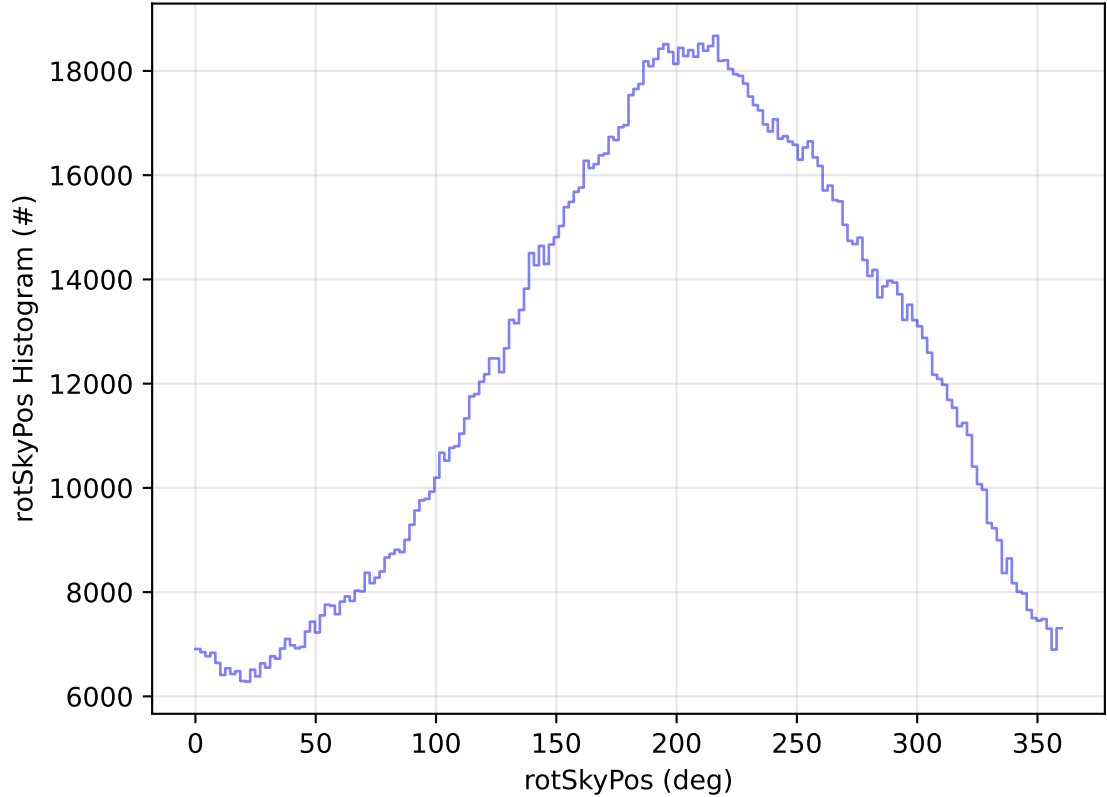
roll_uniform_early_half_accordion1_mjdp0_v3.4_10yrs WFD all bands: rotSkyPos Histogram
