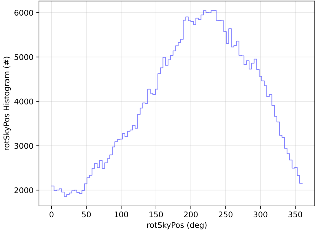
roll_uniform_early_half_accordion1_mjdp0_v3.4_10yrs All sky y band: rotSkyPos Histogram
