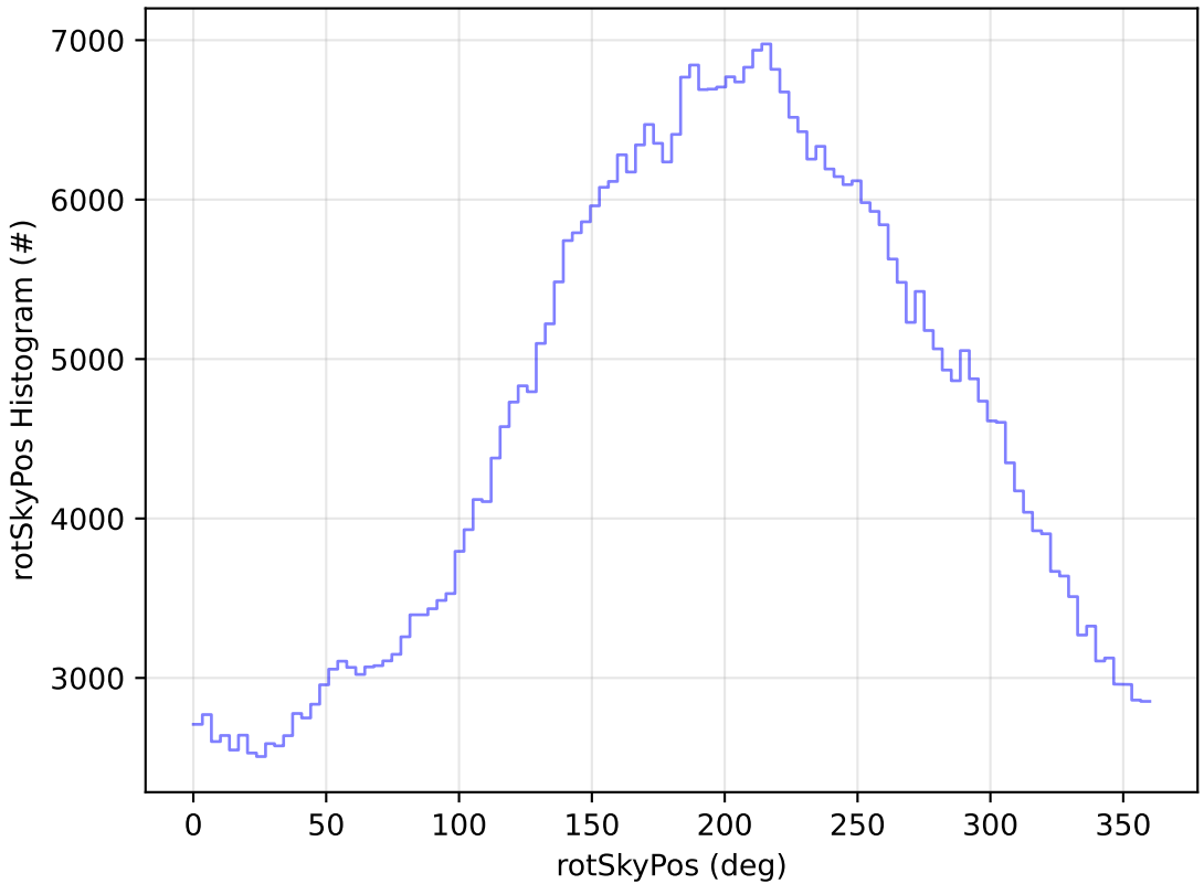
roll_uniform_early_half_accordion1_mjdp0_v3.4_10yrs All sky r band: rotSkyPos Histogram
