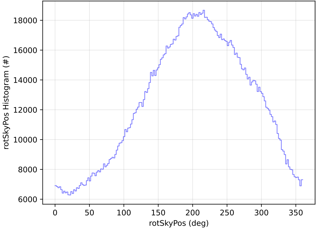
roll_uniform_early_half_accordion1_mjdp0_v3.4_10yrs All sky all bands: rotSkyPos Histogram
