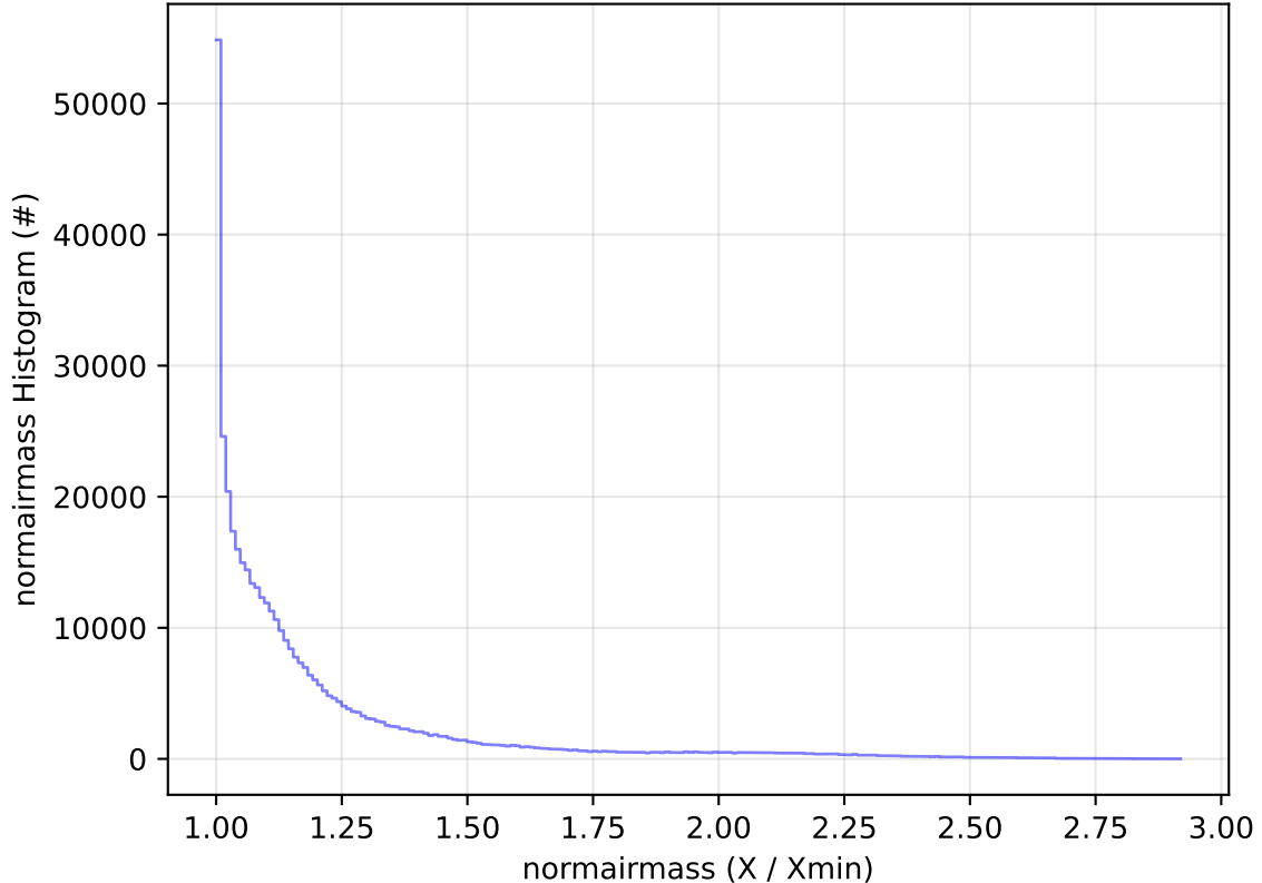
roll_uniform_early_half_accordion1_mjdp0_v3.4_10yrs WFD z band: normairmass Histogram
