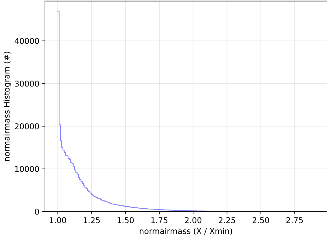
roll_uniform_early_half_accordion1_mjdp0_v3.4_10yrs WFD y band: normairmass Histogram
