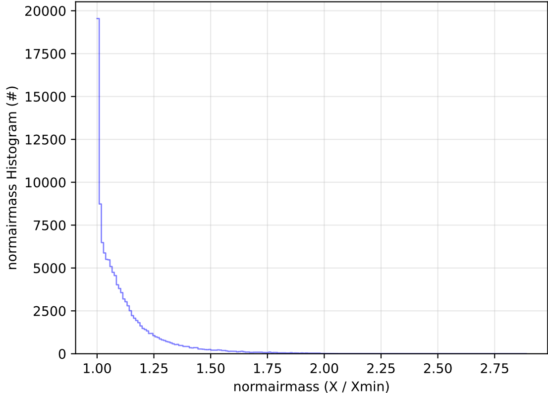
roll_uniform_early_half_accordion1_mjdp0_v3.4_10yrs WFD u band: normairmass Histogram
