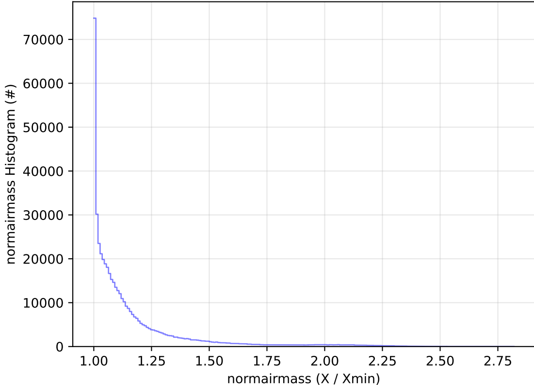
roll_uniform_early_half_accordion1_mjdp0_v3.4_10yrs WFD r band: normairmass Histogram
