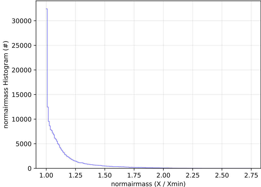
roll_uniform_early_half_accordion1_mjdp0_v3.4_10yrs WFD g band: normairmass Histogram
